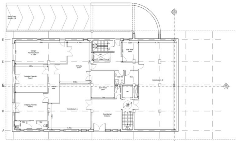
2 Proposed Level -01 Plan Scale 1:100 Built-up Area - 500m 2
