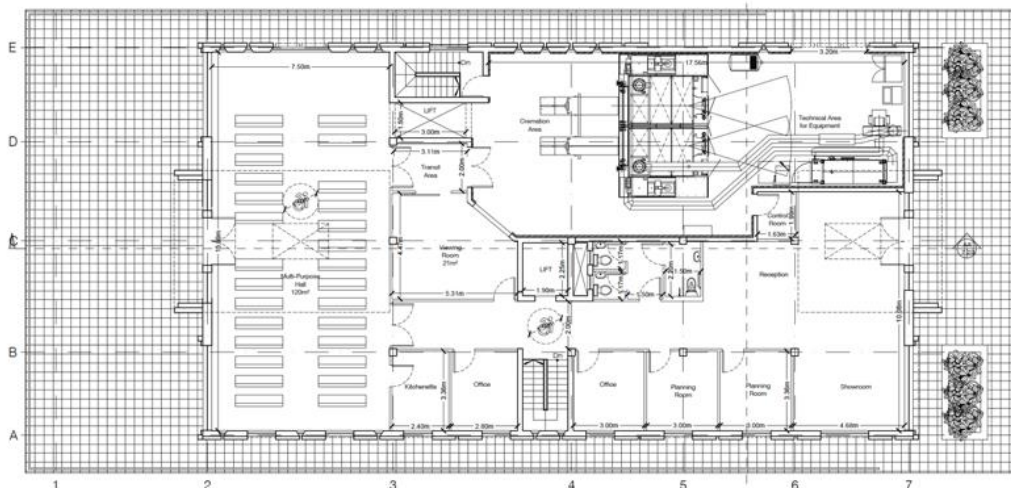
1 Proposed Level 00 Plan Scale 1:100 Built-up Area - 500m 2
